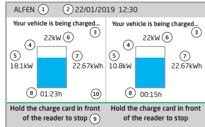
Figure 1b: Display of Eve Double Pro-line during charging with two sockets
