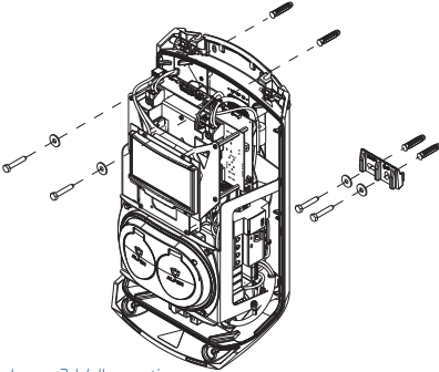
Image 3: Wall mounting
