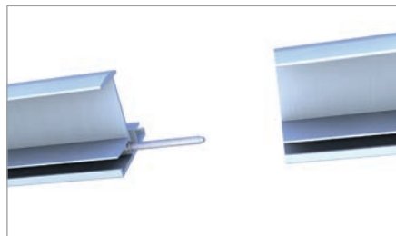
Connecting insertion rails on trapezoidal sheet
