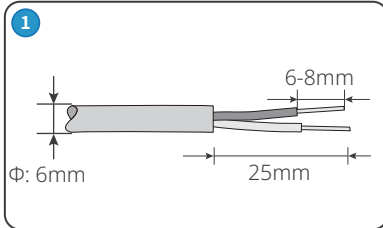
Communication Cable (PIN terminal)
